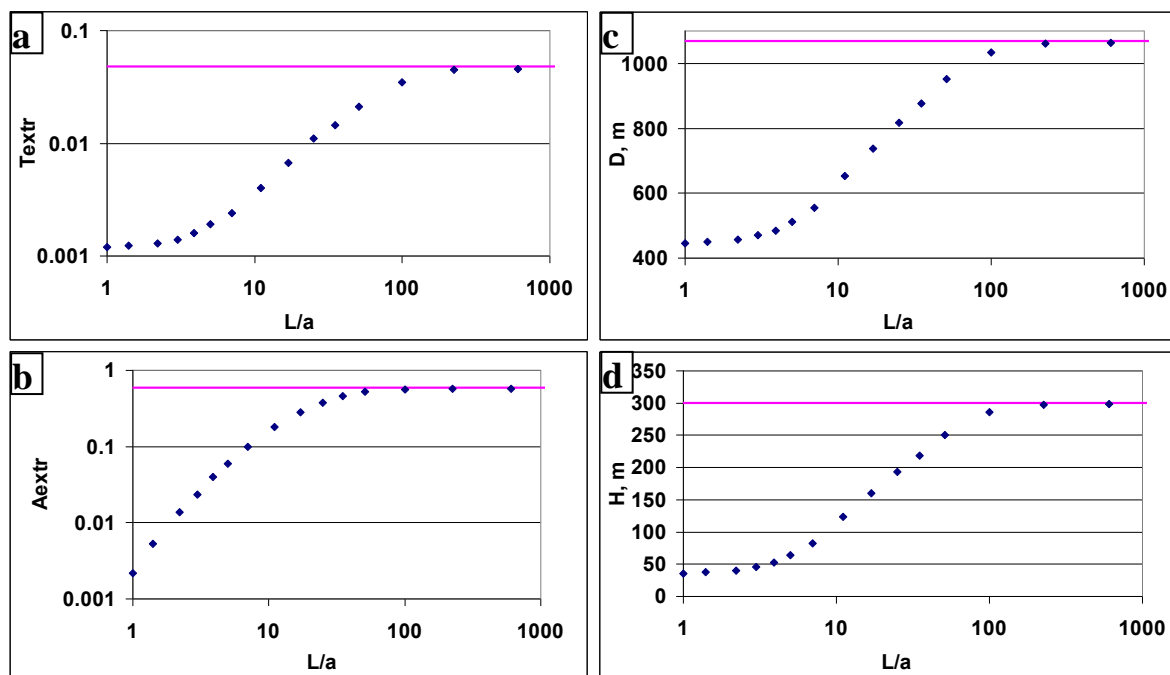
Figure 5. Proportional correlation of the characteristic values on the tipper cross-sections: Text_r (a), A_{extr} (b), D (c) and calculated depth of the body (d) to the values of L/a . Assessment of the body's center depth using the formula for the 2-D case (d). Line shows the values for the 2-D case.
