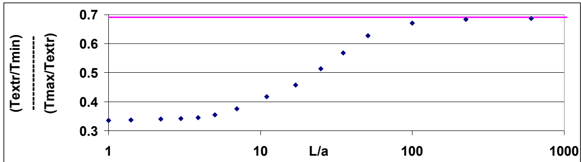
Figure 4. Proportional correlation of the characteristic periods ( P -parameter) on the isometric line 0.5 from A_{extr} to the relative length ( L/a ). P volume for 2-D case is shown by line.
